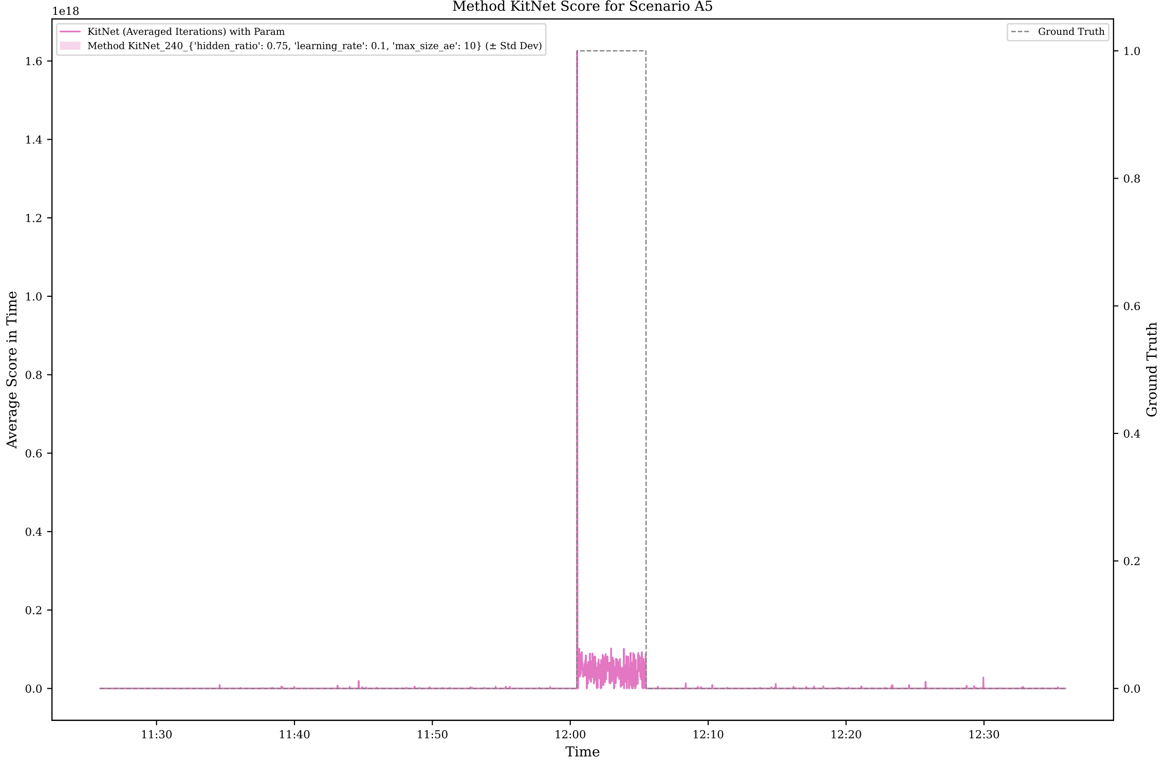
Method KitNet Score for Scenario A5
